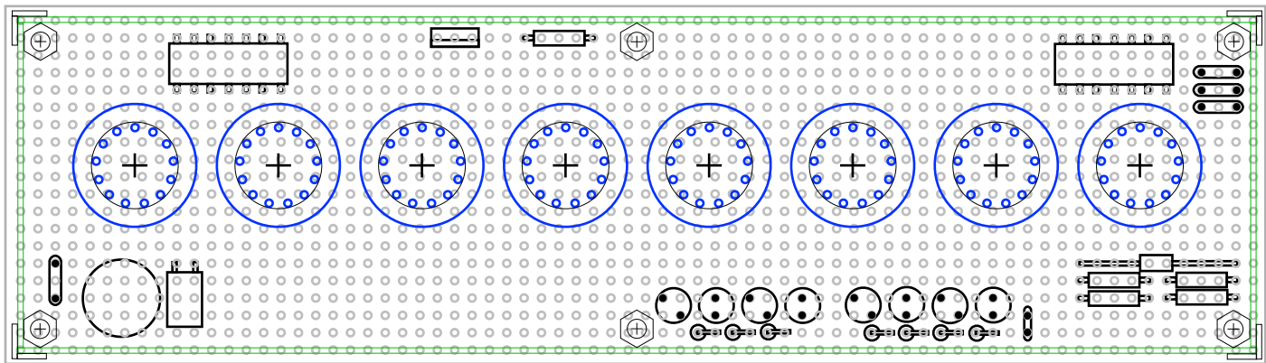
Case method 2 using hex posts. Marked for drilling 1/2" holes for tubes leads.
